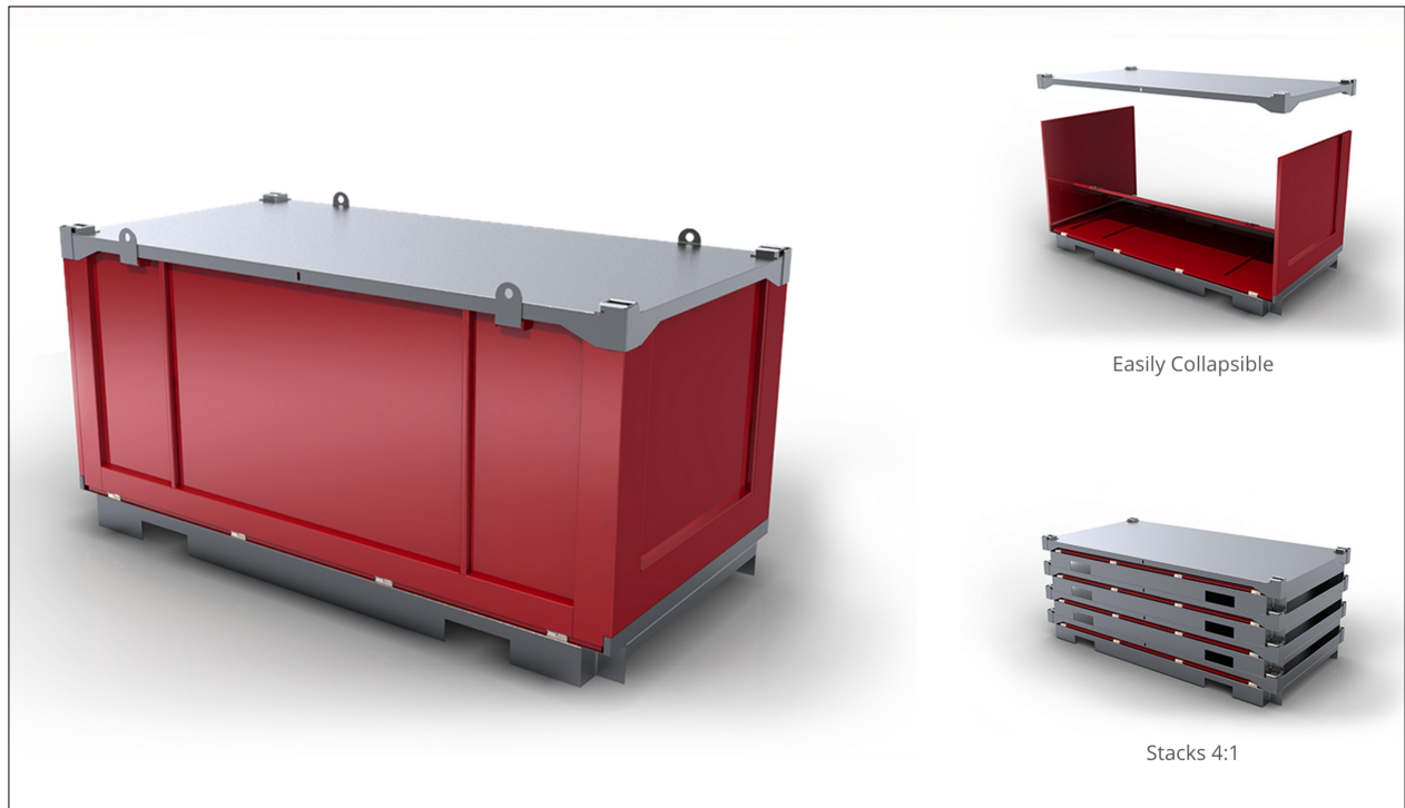
Figure 20. Autobox: an example of container with some desired characteristics of T-containers
